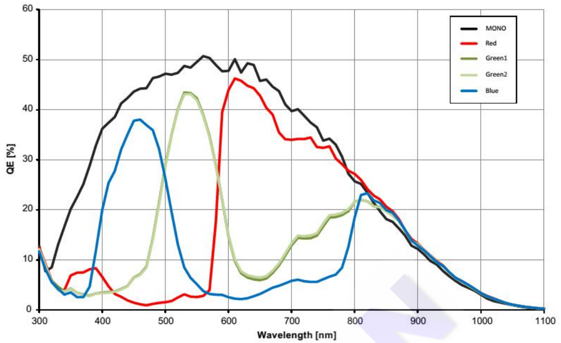
Quantum Efficiency
