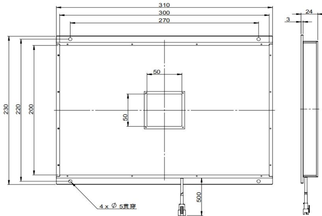
YS-FLK200300 www.yvsion.com
